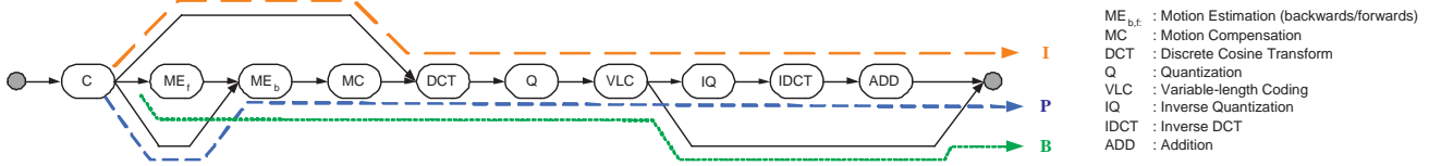
Figure 6. Task graph of the MPEG-2 encoder showing processing of different frame types.
