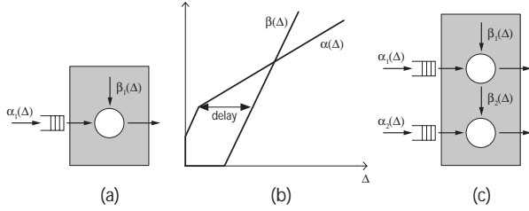
Figure 8. Abstraction of stream processing (a), calculation of the upper bound on the processing delay (b) and abstraction of fixed-priority scheduling (c).
