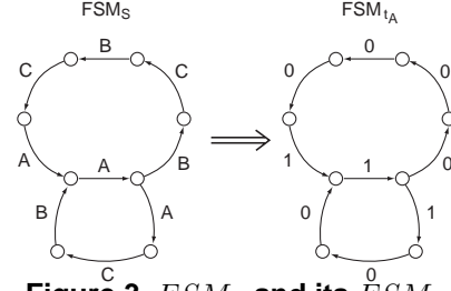
Figure 3. FSM_S and its FSM_{t_A} .
