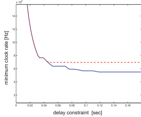
Figure 11. The minimum clock rate computed with type rate curves (solid line) and without using them (dashed line)
