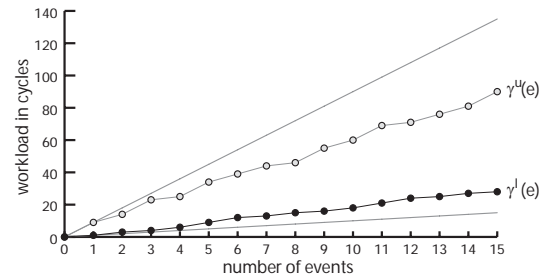
Figure 4. The workload curve for the event stream of Example 1.
