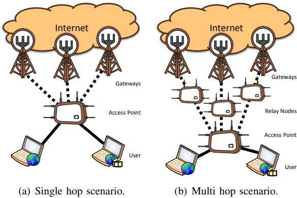
Fig. 1. Scenarios under study.
