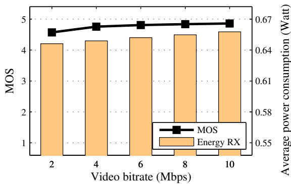
Fig. 6. HD video streaming average power consumption and MOS.
