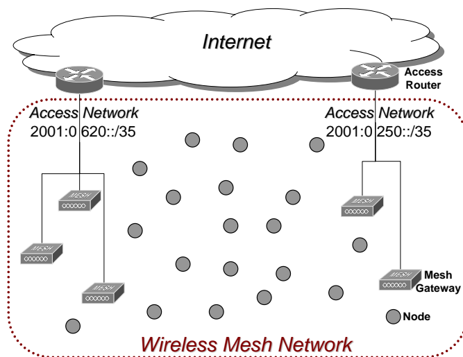
Fig. 1. A wireless mesh network which is connected to the Internet through different access networks.
