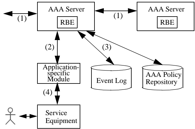
Figure 6: AAA Architecture
