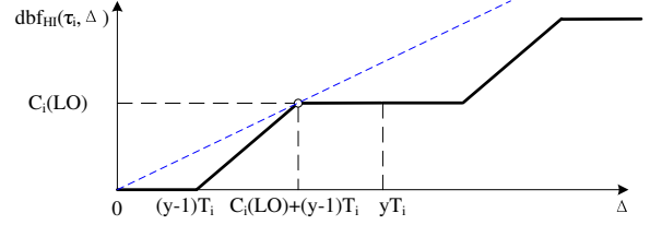
Fig. 3. Approximation of \text{dbf}_{\text{HI}}(\tau_i, \Delta) , \chi_i = \text{LO}
