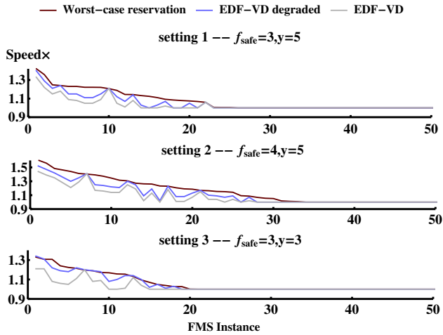
Fig. 6. Processor speedup factors comparison
