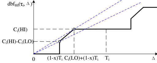
Fig. 2. Approximation of \text{dbf}_{\text{HI}}(\tau_i, \Delta) , \chi_i = \text{HI}
