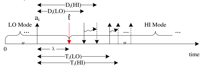
Fig. 1. A mode transition triggered by task overrun
