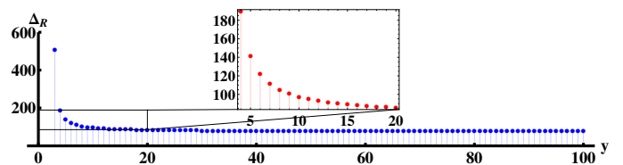
Fig. 5. Trade off between \Delta_R and y
