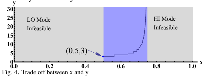
Fig. 4. Trade off between x and y
