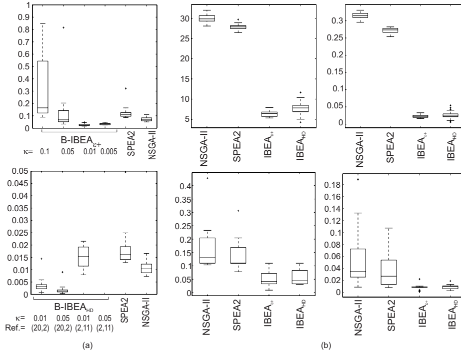
Fig. 2. (a) (top) The indicator values I_{\epsilon_+} for SPEA2, NSGA-II and B-IBEA _{\epsilon_+} for different values of \kappa . For all the different algorithms one outlier was removed from the result sample for improved readability. (bottom) The indicator values I_{HD} for SPEA2, NSGA-II and B-IBEA _{HD} for different values of \kappa and the reference point. In the 4 th column, no values are given because they are about 10 times greater than the values given. (b) Performance comparison for adaptive IBEA _{\epsilon} , IBEA _{HD} , SPEA2 and NSGA-II solving problems DTLZ6 (top) and EXPO2 (bottom). On the left, values for I_{\epsilon_+} , on the right for I_{HD} are given.
