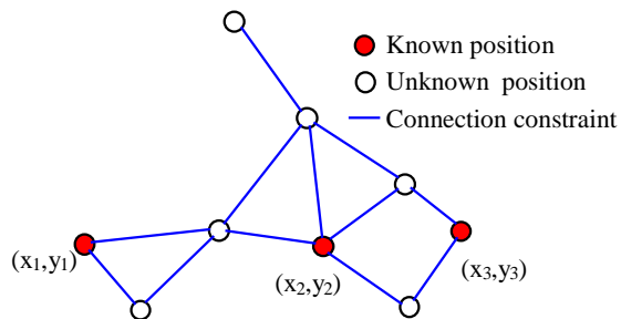
Figure 1. Graph illustrating data and variables as vertices, constraints as edges.
