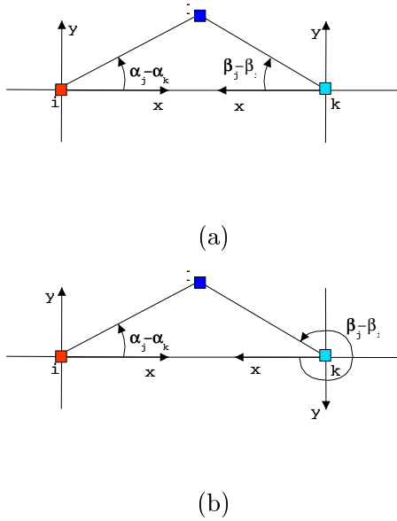
Figure 6. The position of the node j in the Local Coordinate Systems of i and k gives to node k the information whether its coordinate systems needs to be rotated (a) or rotated and mirrored (b).
