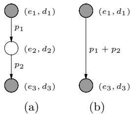
Figure 2: (a) A task graph where vertices 1 and 3 are implemented on processor P and vertex 2 on processor P' , (b) The subgraph seen by processor P
