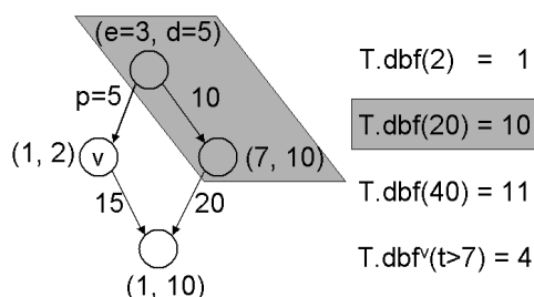
Figure 3: Demand-bound function for task graph T
