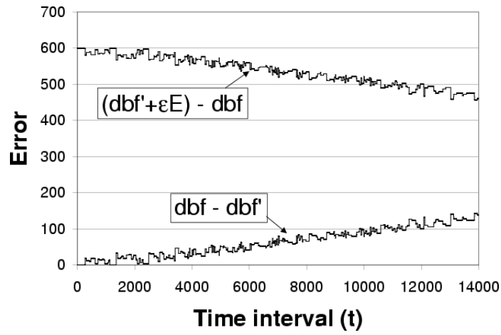
Figure 8: The errors incurred in approximating T.dbf(t) for the example shown in Figure 7
