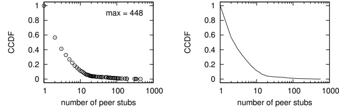
(a) Original distribution of 19,036 peer-degrees in the measured AS topology. (b) Continuous distribution approximating the original one.
