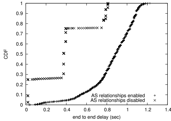
Fig. 2. CDF of e2e delay between traffic sources and destination.
