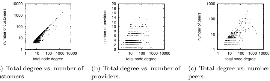
Fig. 8. Scatterplots demonstrating the diversity of annotation degrees and that total node degrees are agnostic with respect to annotations.
