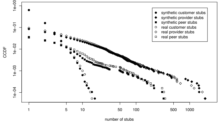
Fig. 6. CCDFs of the number of customer, provider, and peer stubs in the synthetic versus measured AS topology.
