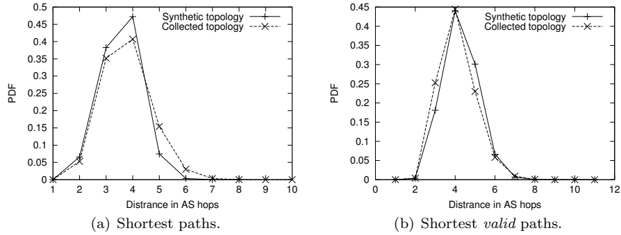
Fig. 7. Distance distributions in synthetic and measured AS topologies.
