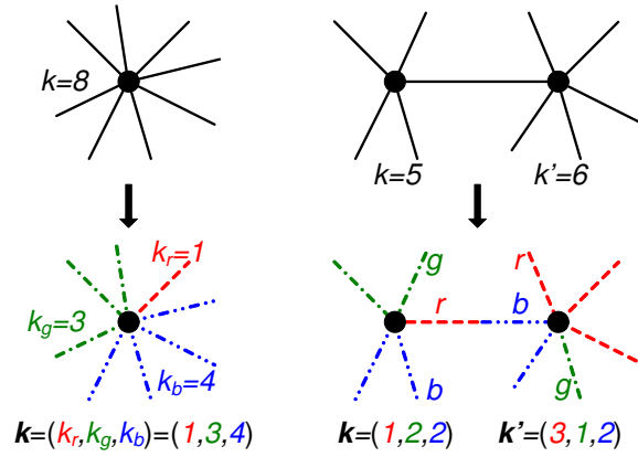
Fig. 3. The 1K- and 2K-annotations. Three different stub colors are represented by dashed (color red), dash-dotted (color green), and dash-double-dotted (color blue) lines.
