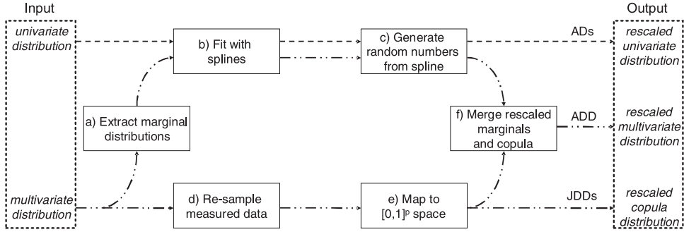
Fig. 5. Overview of rescaling univariate and multivariate distributions.
