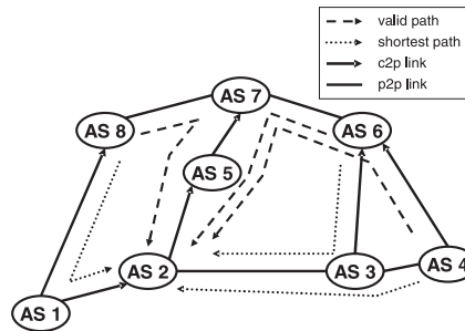
Fig. 1. Example AS topology annotated with AS relationships. The dotted lines represent shortest paths between ASs 4, 6 and 8 to AS 2. The dashed lines represent policy compliant paths from the same sources to the same destination.
