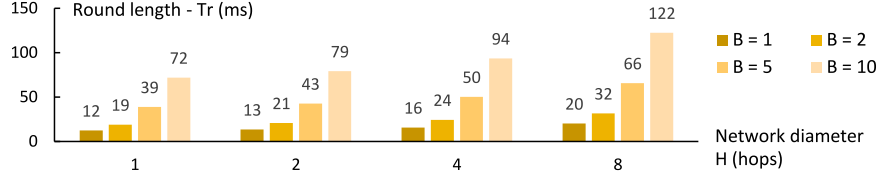
Fig. 6. Sample values of the round length T_r for different network diameters and numbers of slot per round. Payload is l = 10 B and N = 2 .
