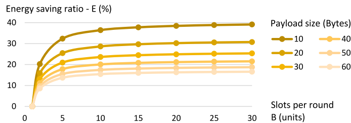
Fig. 7. Relative radio-on time benefit of using rounds compared to single messages. H = 4 , N = 2 . As each round requires only one beacon from the host, the benefit of using rounds grows with the number of number of slots per round (X-axis). Conversely, those savings become less significant as the payload size increases (lighter colors).
