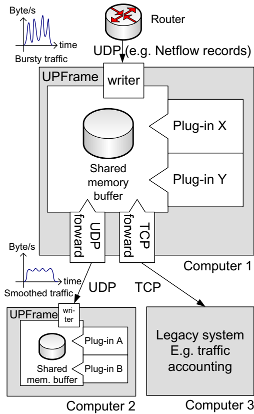
Figure 2. UPFrame architecture
