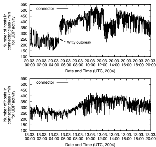
Figure 9. The Witty outbreak significantly raises the number of connecting hosts compared to the previous Saturday.
