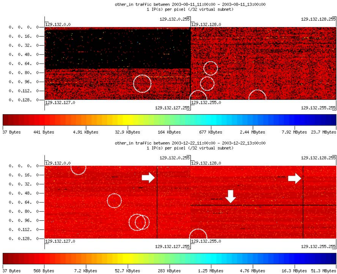
Figure 8. Normal vs. Nachi ICMP incoming network activity
