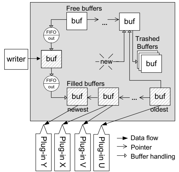
Figure 3. UPFrame buffer handling
