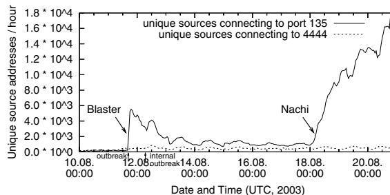
Figure 7. Blaster and Nachi worm outbreaks
