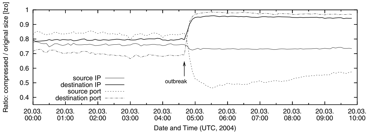
Figure 10. The Witty outbreak clearly changes the compressibility-ratio graphs
