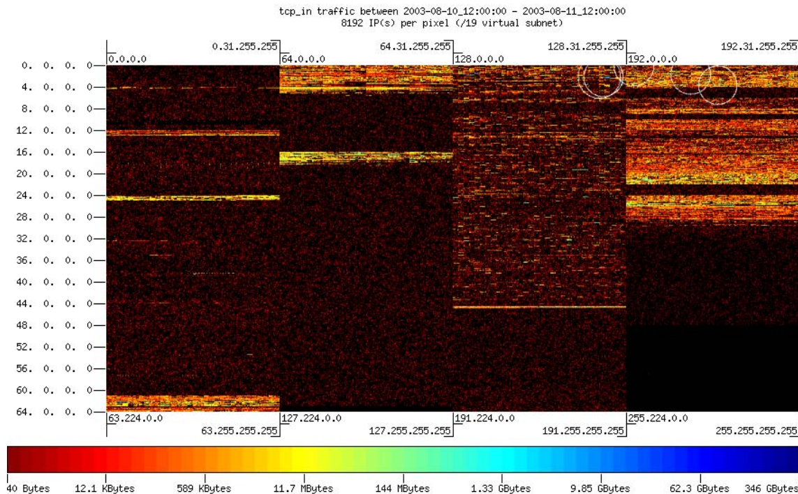
Figure 6. Total TCP inbound traffic for one day as seen in the SWITCH network. The 5 most active hosts are highlighted with a white circle.
