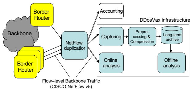
Figure 1. SWITCH network and DDoSVax infrastructure
