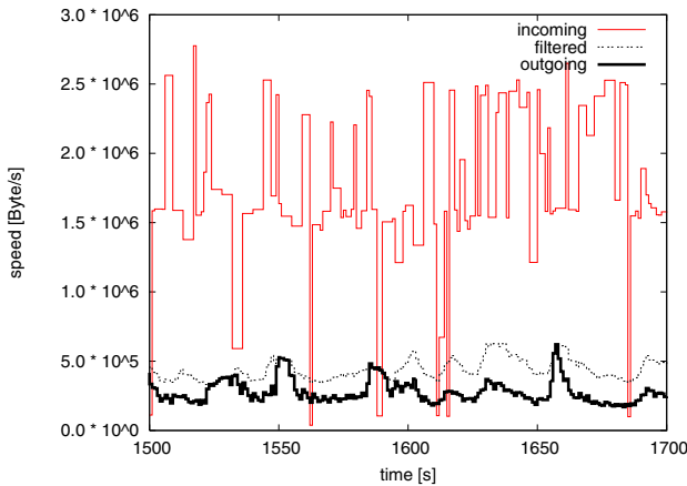
Figure 4. UPFrame traffic shaping
