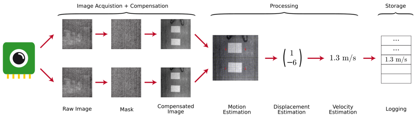
Fig. 1: Overview of the proposed energy-opportunistic walking speed estimation sensor.
