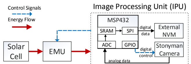
Fig. 2: Architecture of the wearable vision sensor.
