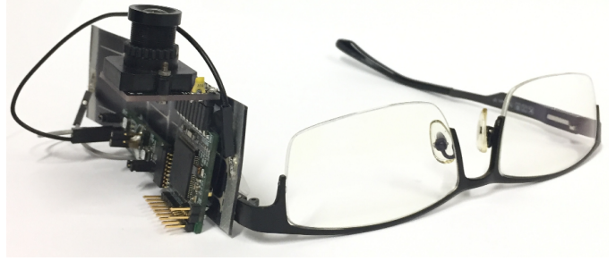
Fig. 3: Image of the wearable, batteryless vision sensor prototype with a flexible solar panel mounted on conventional glasses.
