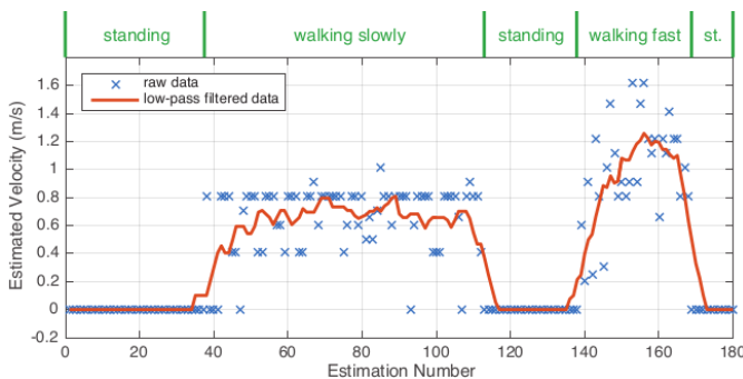
Fig. 5: Velocity of the walking person estimated by the vision sensor prototype (blue crosses) and post-processed in Matlab using a low-pass filter (red line).
