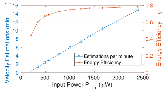
Fig. 4: Measured energy efficiency and execution rate as a function of the input power.
