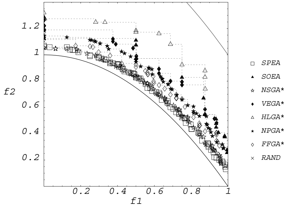
Figure 9: Results on the test function \mathcal{T}_2 using elitism.
