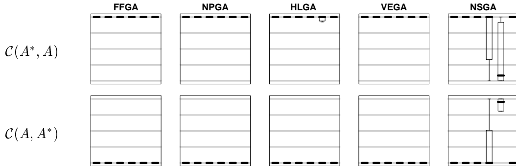
Figure 10: Box plots comparing each non-elitism algorithm A with its elitism-variant A^* .
