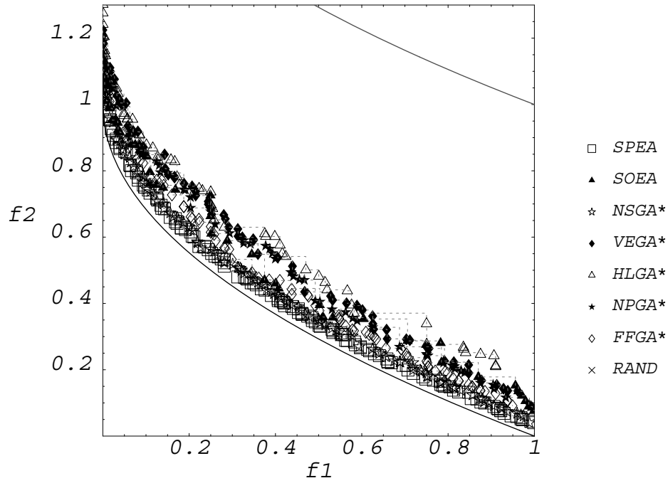
Figure 8: Results on the test function \mathcal{T}_1 using elitism.
